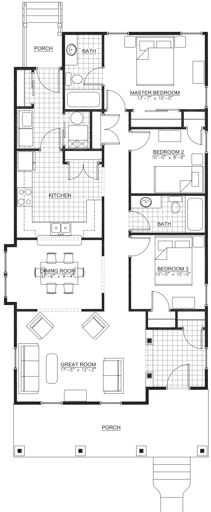
Floor Plan B
