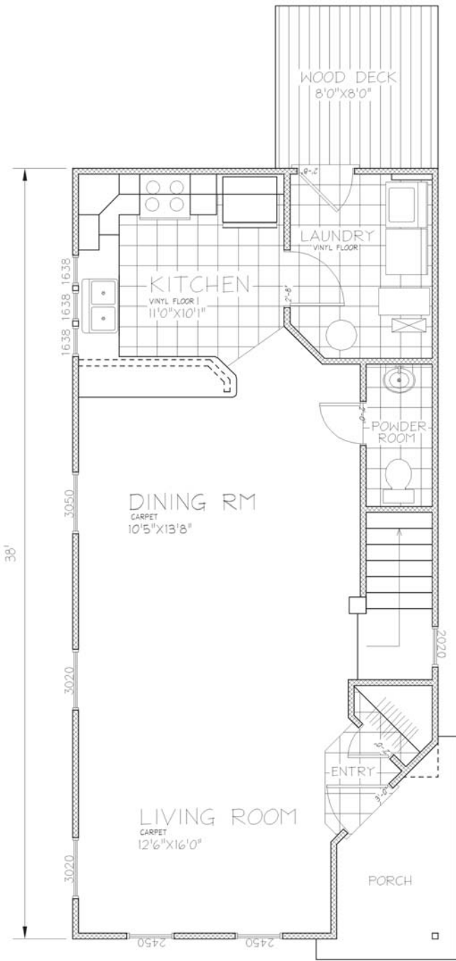
FIRST FLOOR PLAN 648 SQ. FT.
